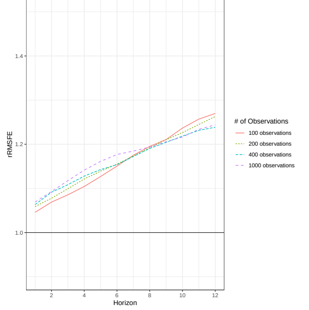
Figure 3: Case 1.1: AR(1) , \alpha = 0.9 , additive transformation
